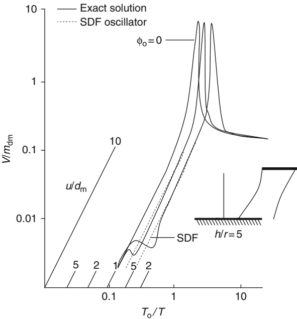
Fig. 6.3 A comparative study of exact and SDF oscillator results ( h/r = 5 )
