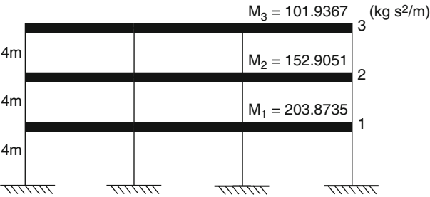
Fig. 9.8 A three bay three-storey frame
