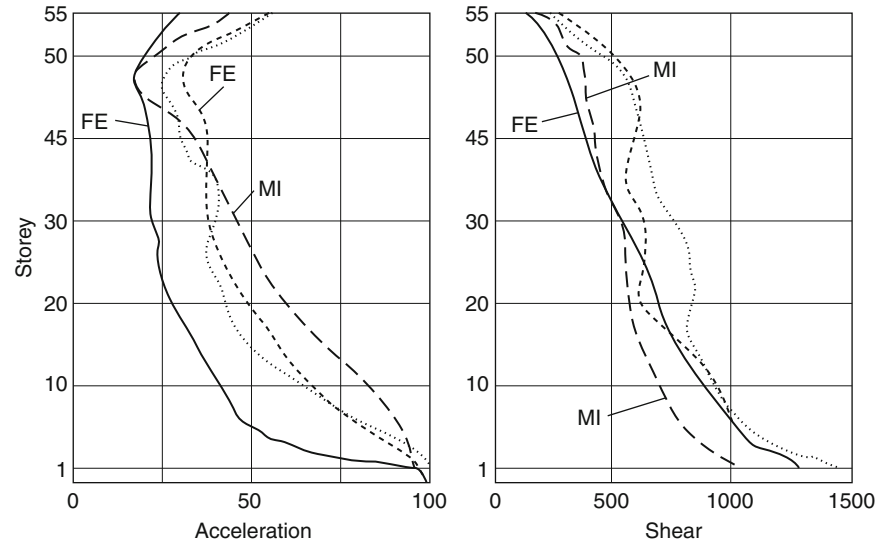
Fig. 7.23 Linear earthquake response-A comparative study FE-Finite Element Analysis By Bangash using El-centro MI-Muto Institute, Japan, using Taft \xi = 3\% damping
