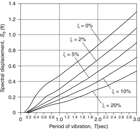
Fig. 4.10 Average displacement response spectrum (El-Centro, 1940) (US Atomic Energy Report TID-7024, August 1963)
