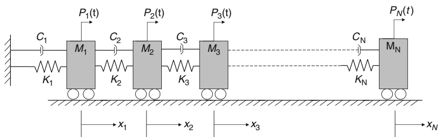
Fig. 3.9 Multi-degree-of-freedom system
