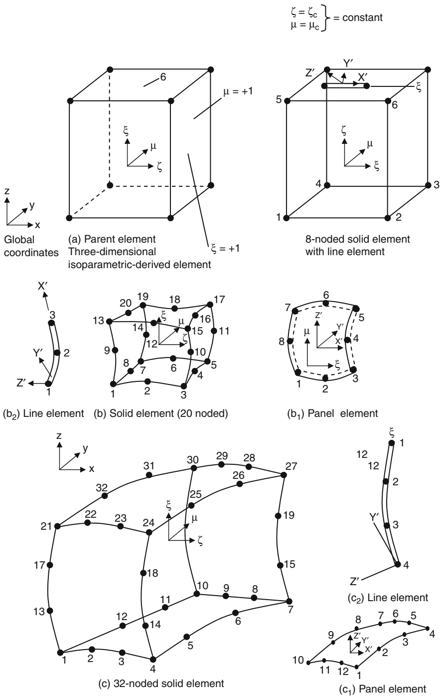
Fig. 5.26 Finite elements
