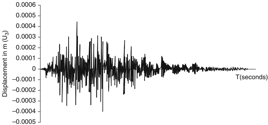
Fig. 5.14 Third-storey response displacement history in physical coordinates
