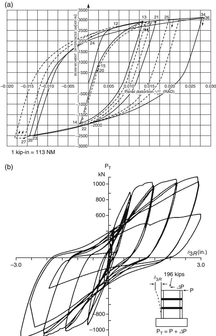
Fig. 4.37 Force-deformation relations
