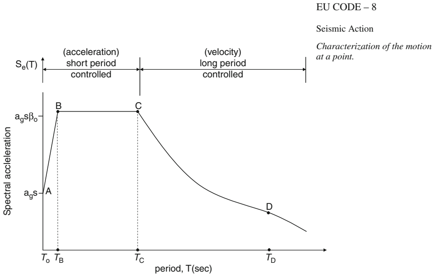
Fig. 9.1 Response spectra
