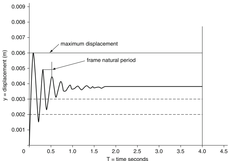
Fig. 4.50 Displacement–time relationship
