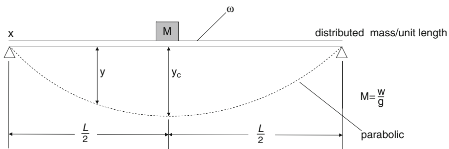
Fig. 3.6 Uniform mass on a beam
