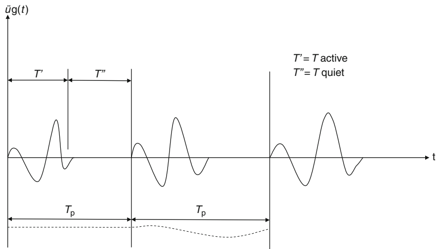
Fig. 6.6 Acceleration–time relationship
