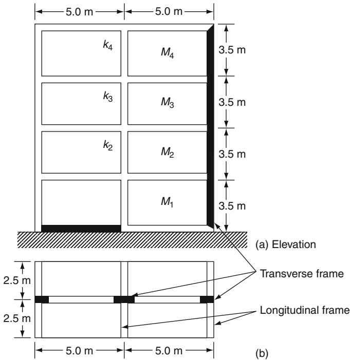
Fig. 4.53 Four-storey building
