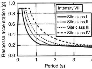
Site spectra for the four kind site classes (China)
