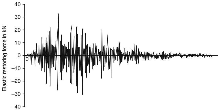
Fig. 5.17 Lateral load response first storey (kN)
