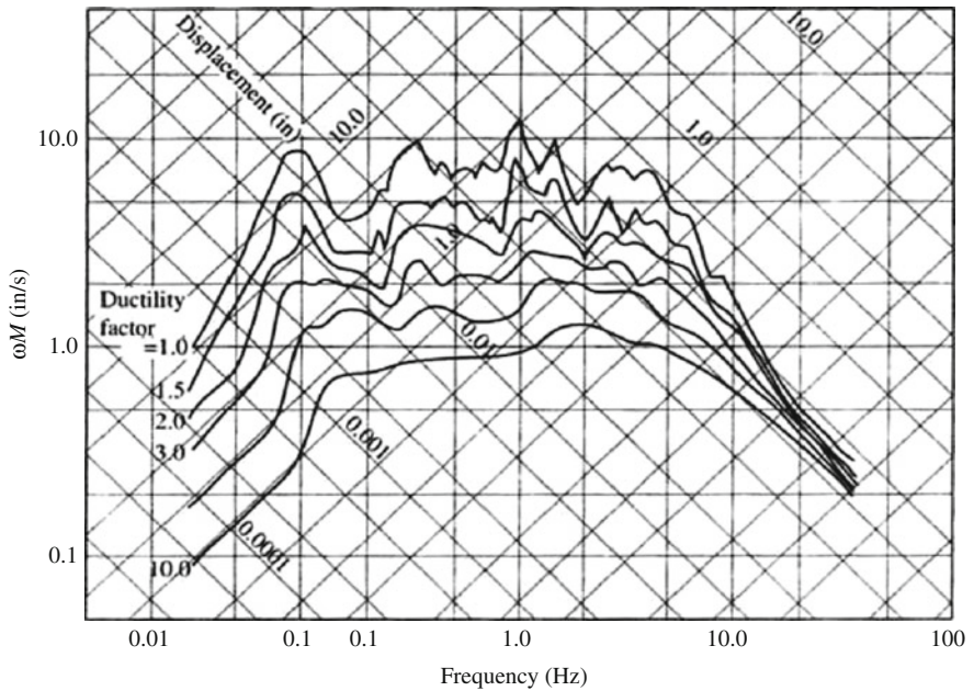
Fig. 6.5 Frequency spectra
