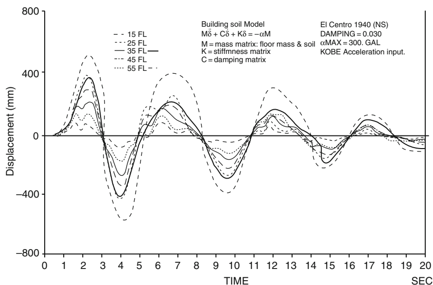
Fig. 7.5 Displacement–time history (Kobe)
