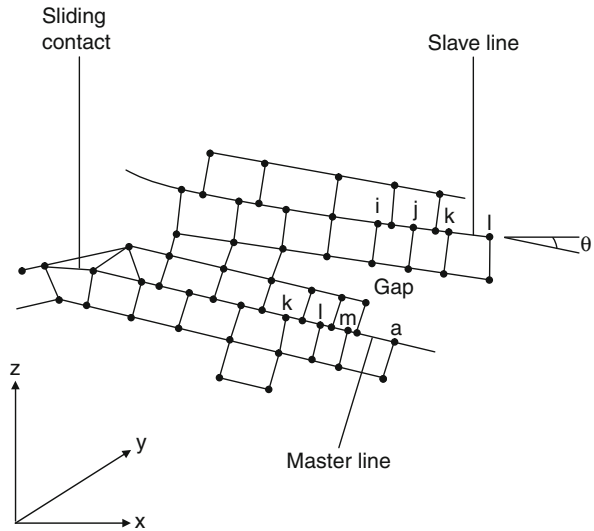
Fig. 5.39 Contact or gap element
