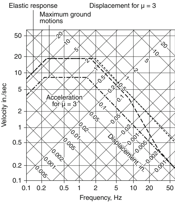
Fig. 4.12 Inelastic design spectra (Newmark and Hall, 1982)
