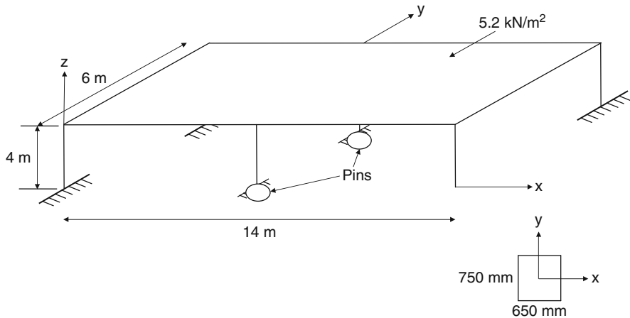
Fig. 9.4 Concrete slab supported by six columns
