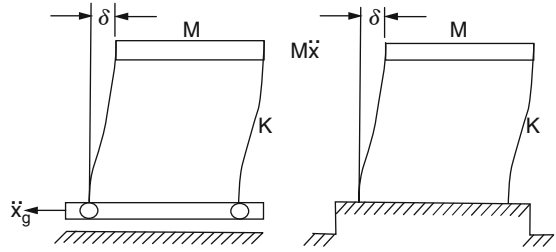
Fig. 4.2 A single-degree-of-freedom oscillator
