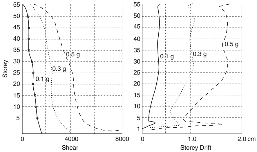
Fig. 7.24 Non-linear earthquake response-A comparative study Intensity marked 0.1, 0.3, 0.5g. Results from F.E. \xi = 3\% damping
